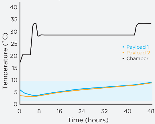
Example: E series, summer ambient data Pack-out Configuration: RBC20M48-M5
