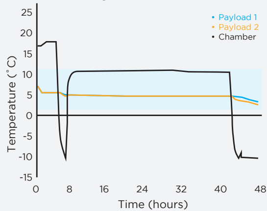
Example: E series, winter ambient data Pack-out Configuration: RBC20M48-M5
